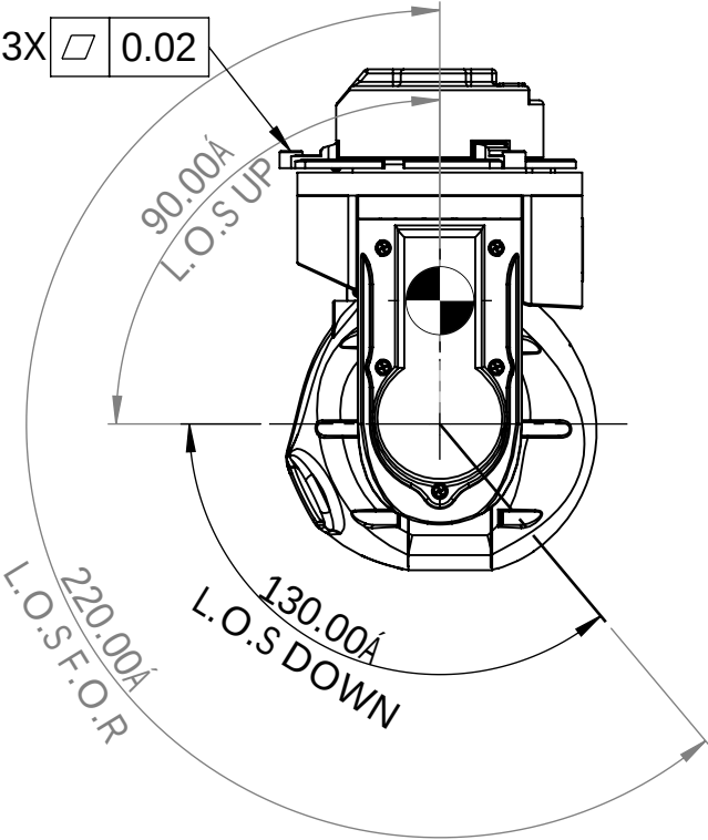
LHS VIEW
